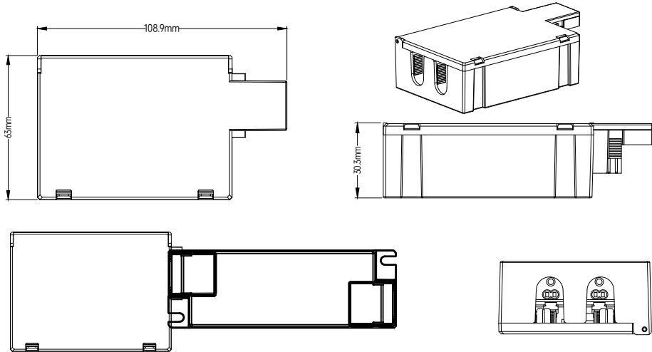
Combined(Side View)
