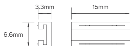
614032 - Connector
