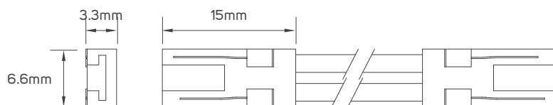
614034 - Connector
