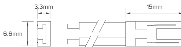
614033 - Connector
